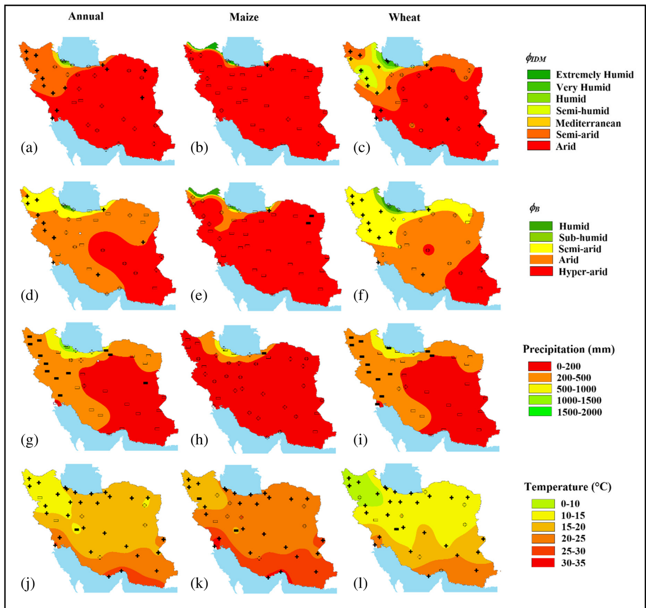
Fig. 2 Spatial distribution of \phi_{IDM} , \phi_B , mean precipitation, and mean temperature over Iran (1966–2015). Plus (+) and minus (–) show the positive and negative trends by MK_O at the 90% confidence level,
