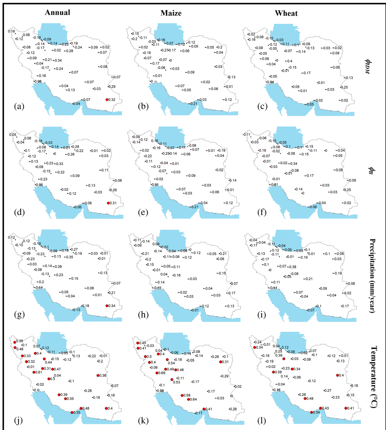
Fig. 3 Spatial distribution of lag-1 serial correlation ( \rho ) of \phi_{DM} , \phi_B , mean precipitation, and mean temperature series over Iran (1966–2015). Red circles show the significant lag-1 serial correlation at the 95% confidence level
