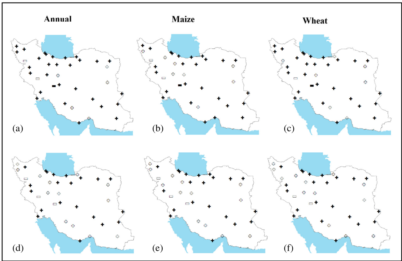
Fig. 6 Spatial distribution of mean temperature Mann–Kendall trend modified by effective sample size method ( MK_{ess} ) (the top row) and long-term persistence method ( MK_{LTP} ) (the bottom row)
