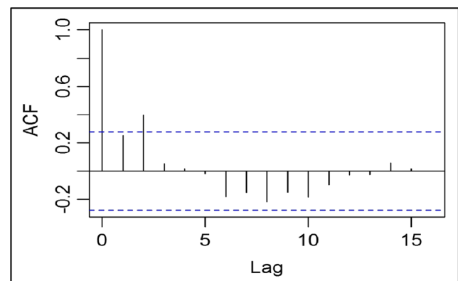
Fig. 5 Autocorrelation function for \phi_{IDM} at wheat growing season at Zahedan station, southeast of Iran
