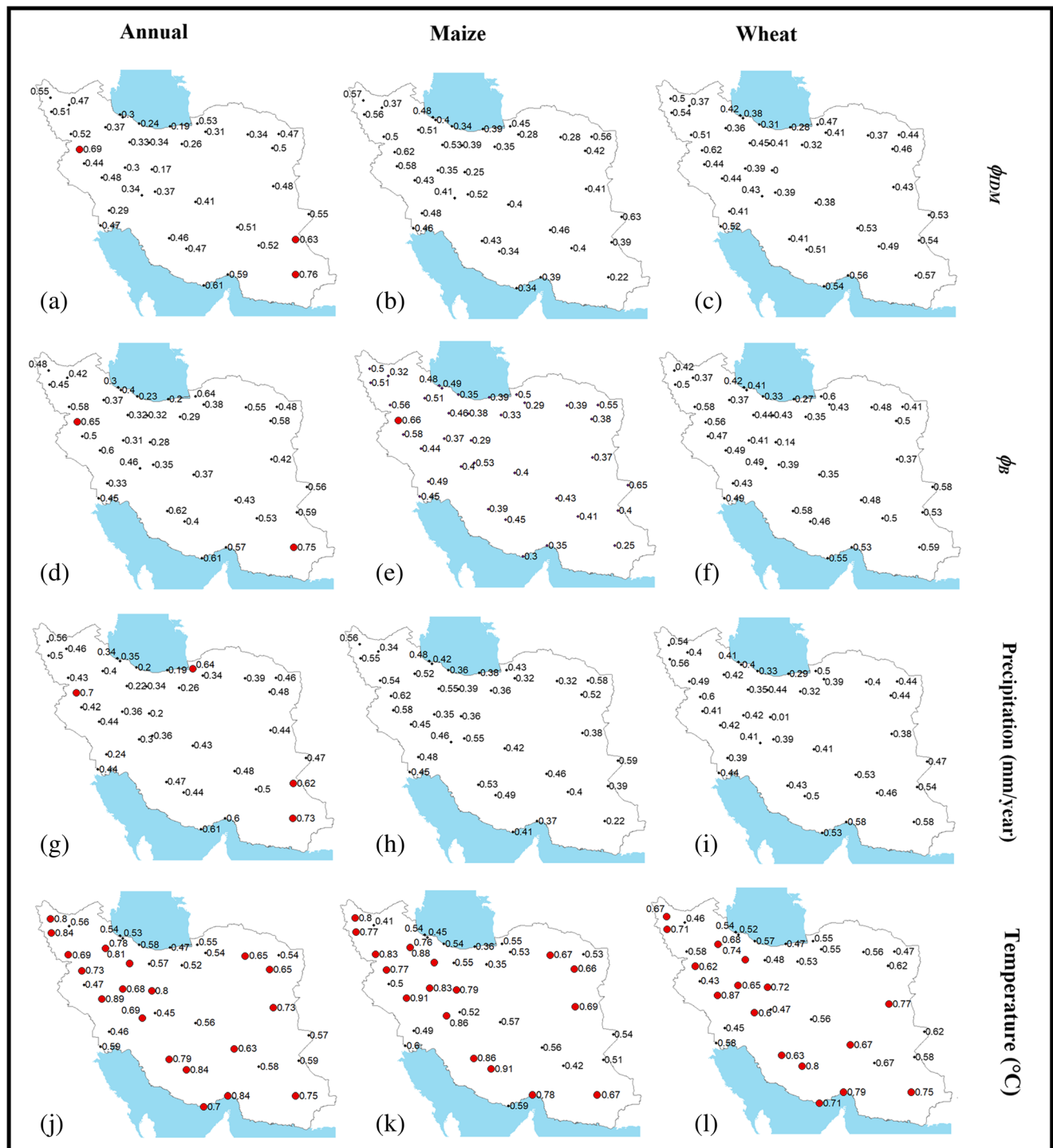
Fig. 4 Spatial distribution of Hurst exponent ( H ) of \phi_{DM} , \phi_B , mean precipitation, and mean temperature series over Iran (1966–2015). Red circles show the significant Hurst exponent at the 95% confidence level
